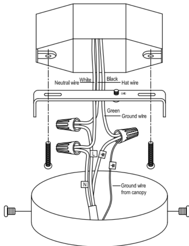
Wire connection diagram
